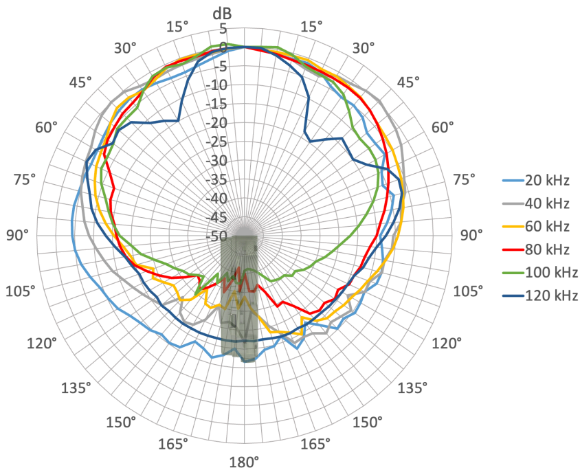
Figure 11. Ultrasonic Microphone Polar Response: Top View
