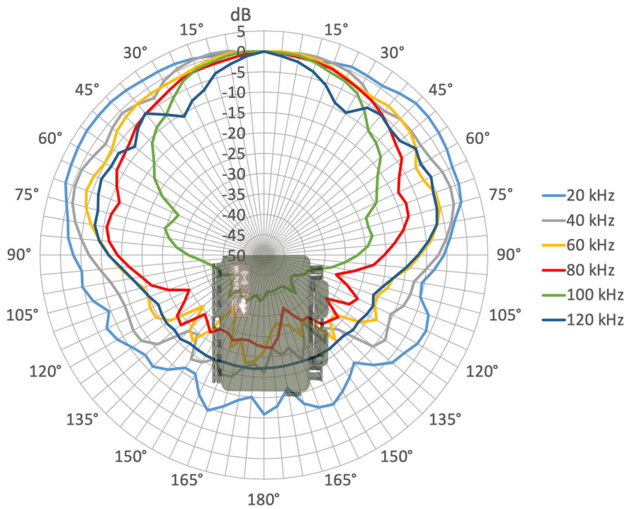
Figure 10. Ultrasonic Microphone Polar Response: Front View
