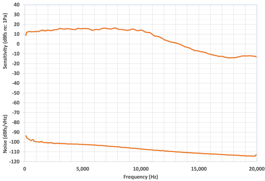
Figure 12. Sensitivity and Noise Floor, Linear Frequency Scale
