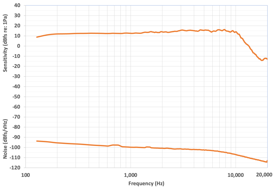
Figure 13. Sensitivity and Noise Floor, Logarithmic Frequency Scale
