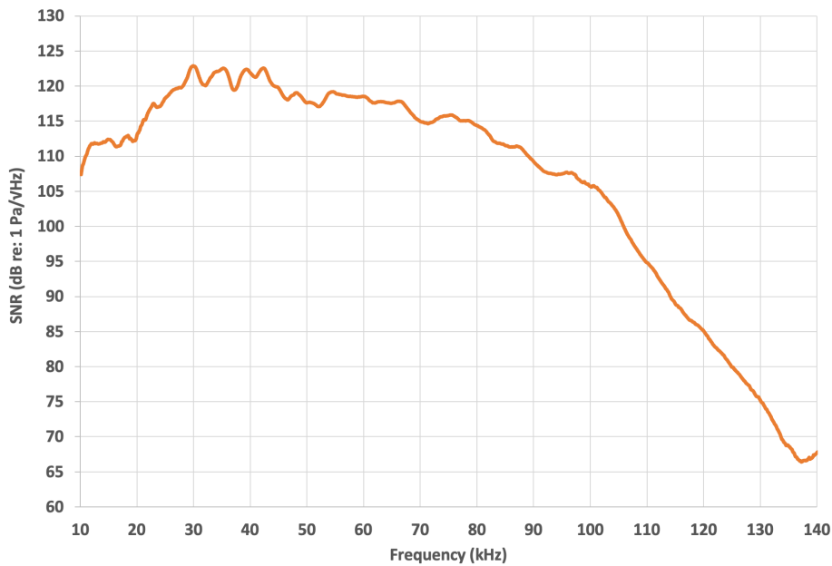
Figure 9. Ultrasonic Microphone Signal-to-Noise Ratio
