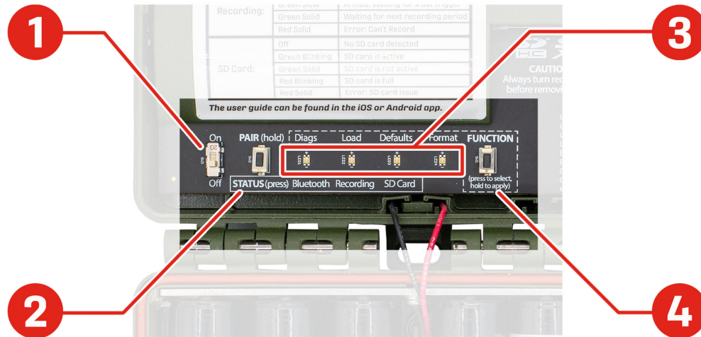
Figure 6. Control Panel
