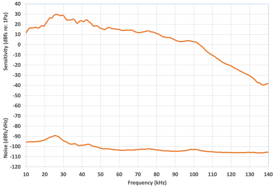
Figure 8. Ultrasonic Microphone Sensitivity and Noise Floor
