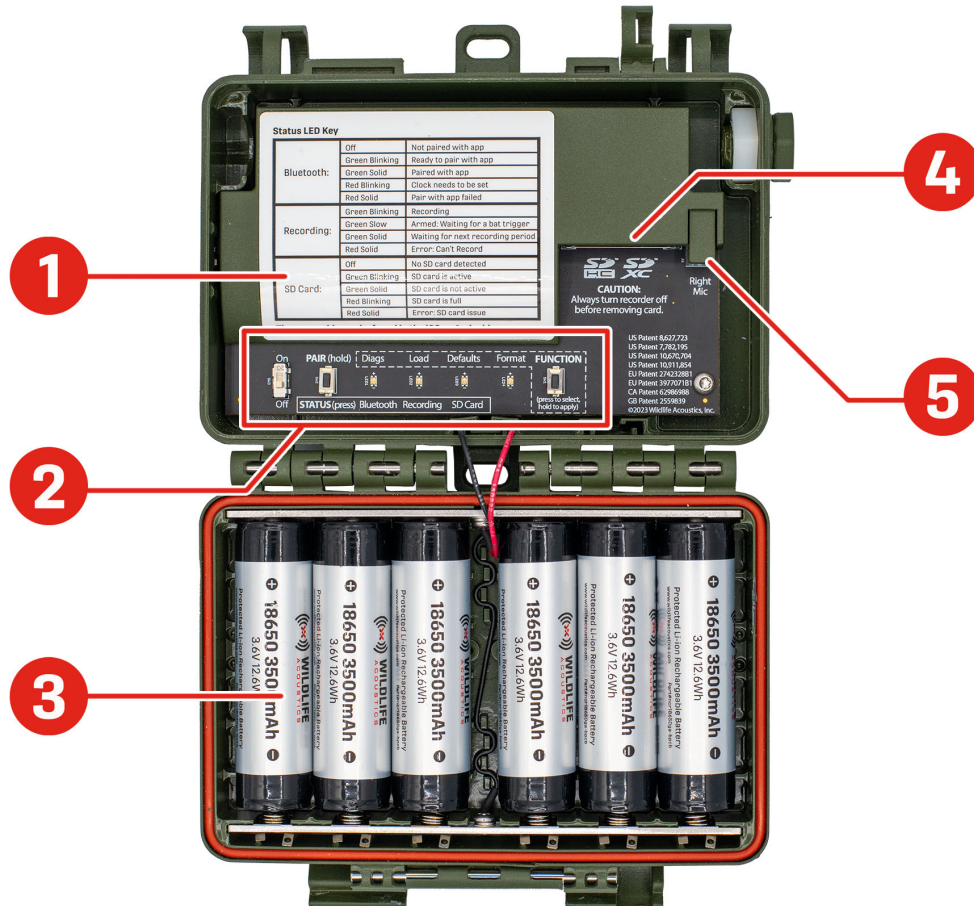
Figure 5. Internal Overview
