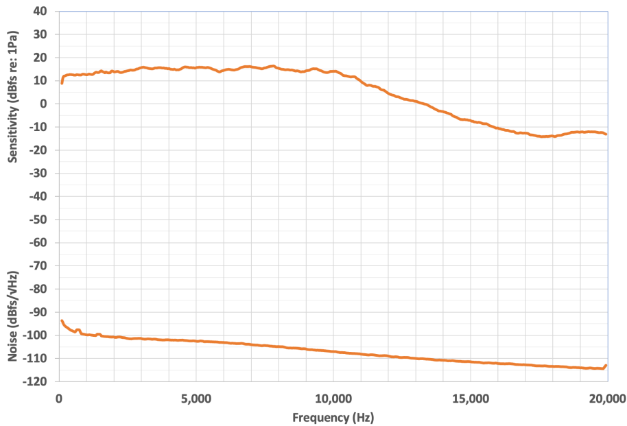
Figure 7. Sensitivity and Noise Floor, Linear Frequency Scale
