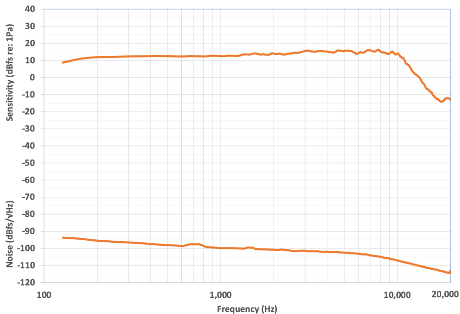
Figure 8. Sensitivity and Noise Floor, Logarithmic Frequency Scale
