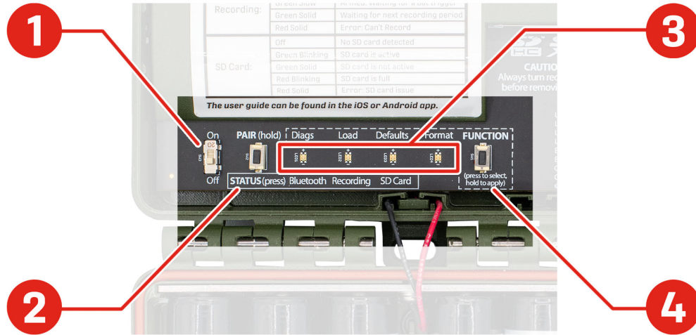
Figure 5. Control Panel
